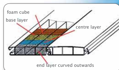
Sealing system
