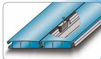
Locking system
